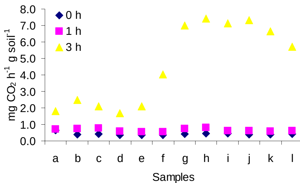
Figure 3.19 Different carbon dioxide measured in twelve different jars (a- l), at different incubation times: 0 h ( \text{CO}_2 measured without sealing the jar); 1 h ( \text{CO}_2 measured after jar had been sealed for one hour); 3 h ( \text{CO}_2 measured after jar had been sealed for three hours).
