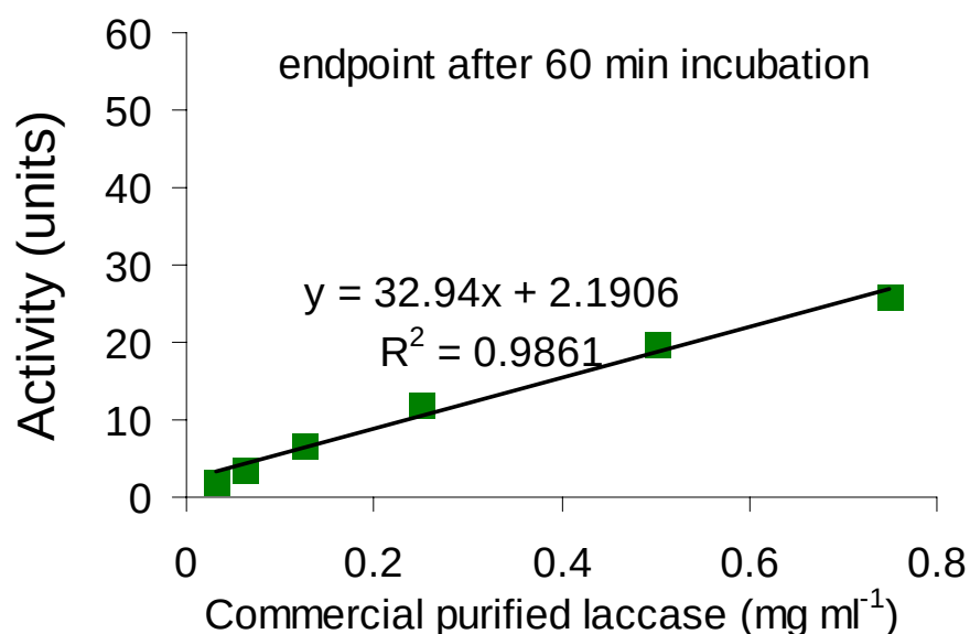
Figure 3.8 Linear regression of laccase activity against concentration of purified commercial laccase from Rhus vernificera . The microtitre plate reader was set in endpoint mode and the microtitre plate was incubated for 60 mins at 37°C.
