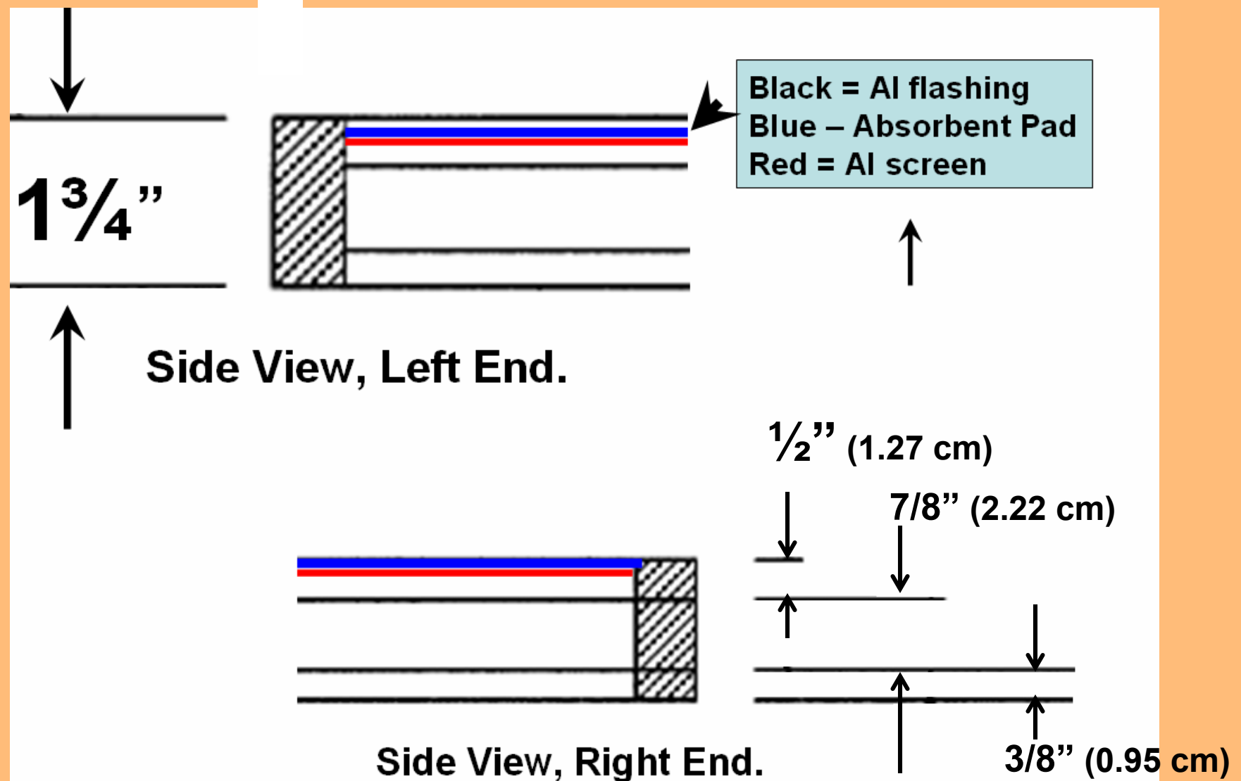
Fig. 4. Side view detail.
