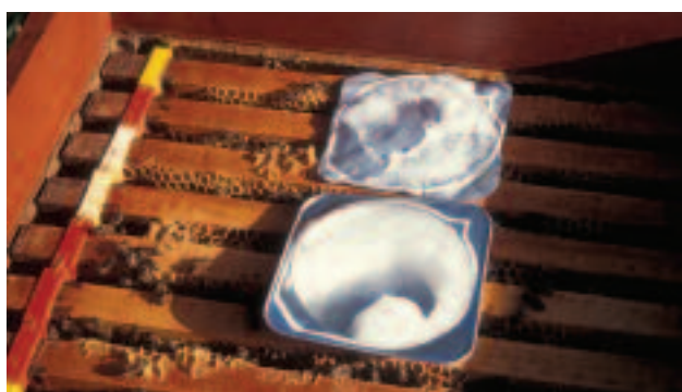
Figures 41 and 42: Apiguard treatments
