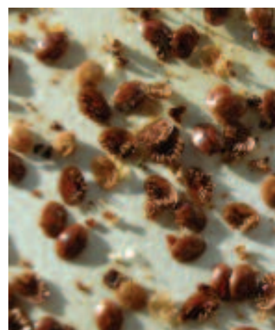
Figure 21: Hive floor debris containing mites
