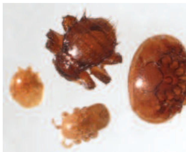
Figure 18: Braula coeca compared to varroa, Tropilaelaps and Melittiphis
