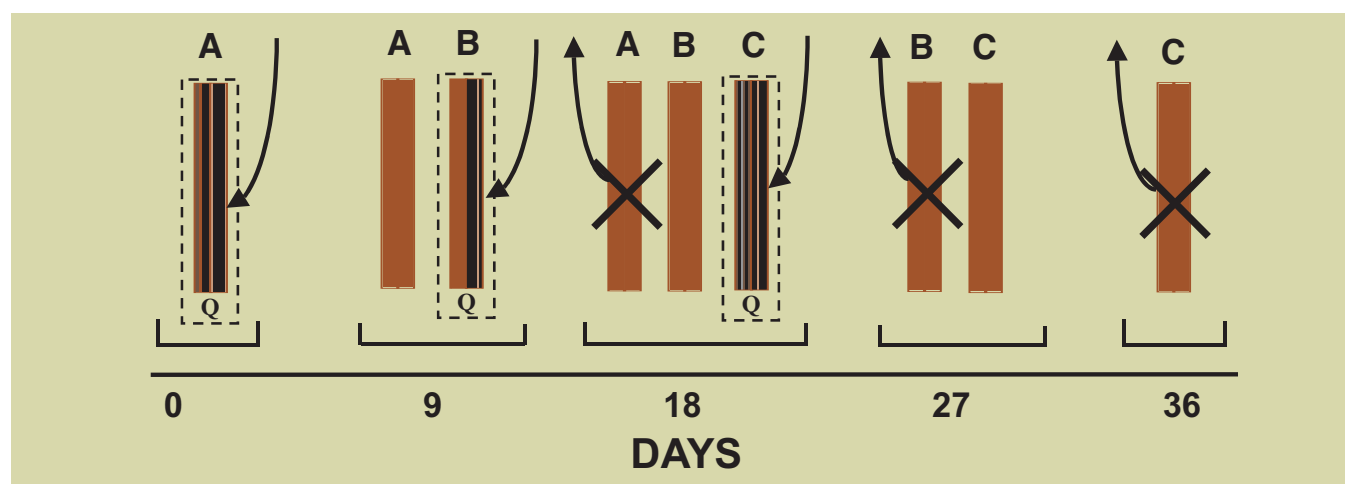
Figure 33: Comb trapping timetable. The queen ('Q') is caged for 9 days on three combs ('A', 'B' and 'C') in succession. These each remain in the colony for a further 9 days while varroa mites enter the brood cells to breed. The combs containing mites 'trapped' in sealed brood are then removed. See 'Comb Trapping' (page 15) for details
