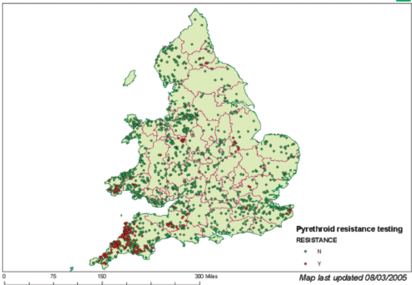
Figure 44: Map showing confirmed pyrethroid resistance in England and Wales (as of March 2005)
