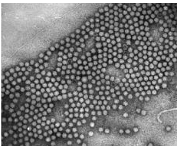
Figure 9: Electron micrograph of particles of Acute Bee Paralysis Virus (ABPV), representative of any 30nm virus particles in bees
