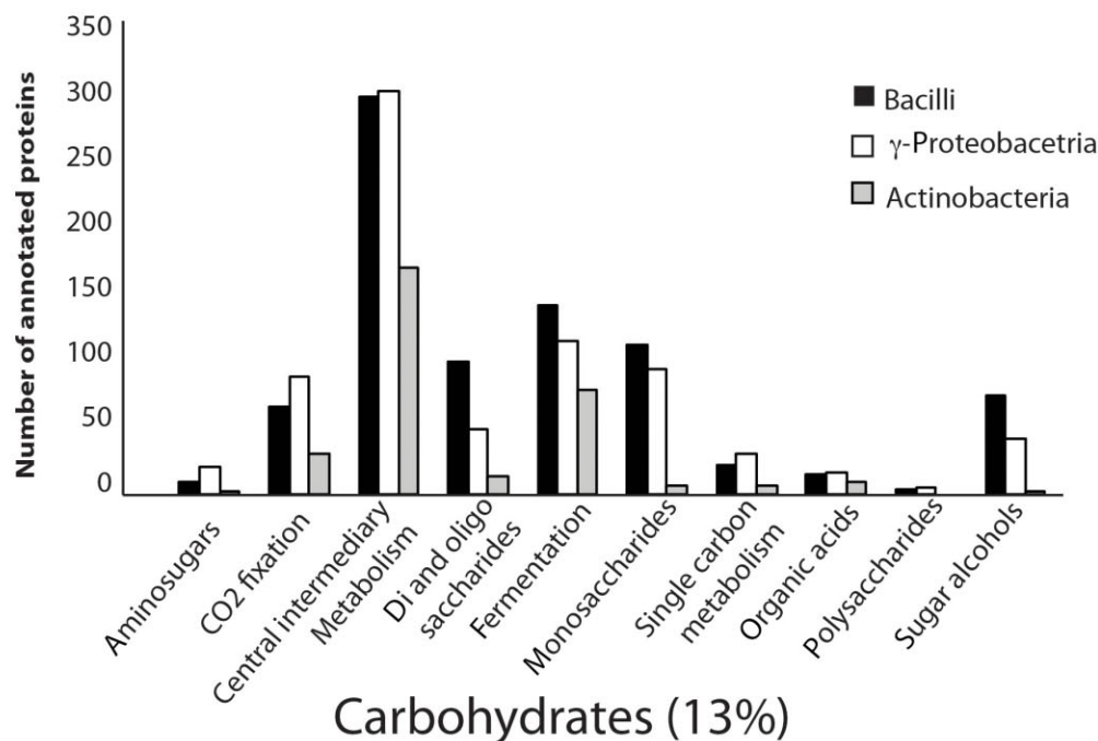
Fig. 2. The second most abundant functional class (based on MG-RAST subsystems hierarchical annotation) of transcripts is carbohydrate metabolism.
