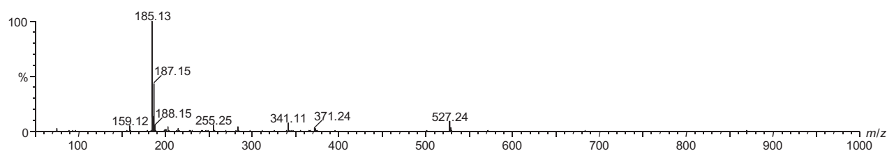
Figure 4 Electrospray ionization mass spectrometry spectrum of RJ 48-h storage at room temperature.
