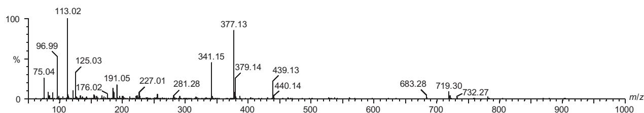
Figure 3 Electrospray ionization mass spectrometry spectrum of royal jelly (AS) adulterated with powered milk.
