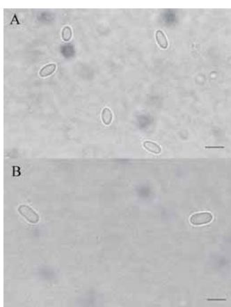
Plate 37: Nosema spores under a light microscope: (a) Nosema apis ; (b) Nosema ceranae Bar=5 \mu m (©ifries; photograph J Apic Res, 2006)
