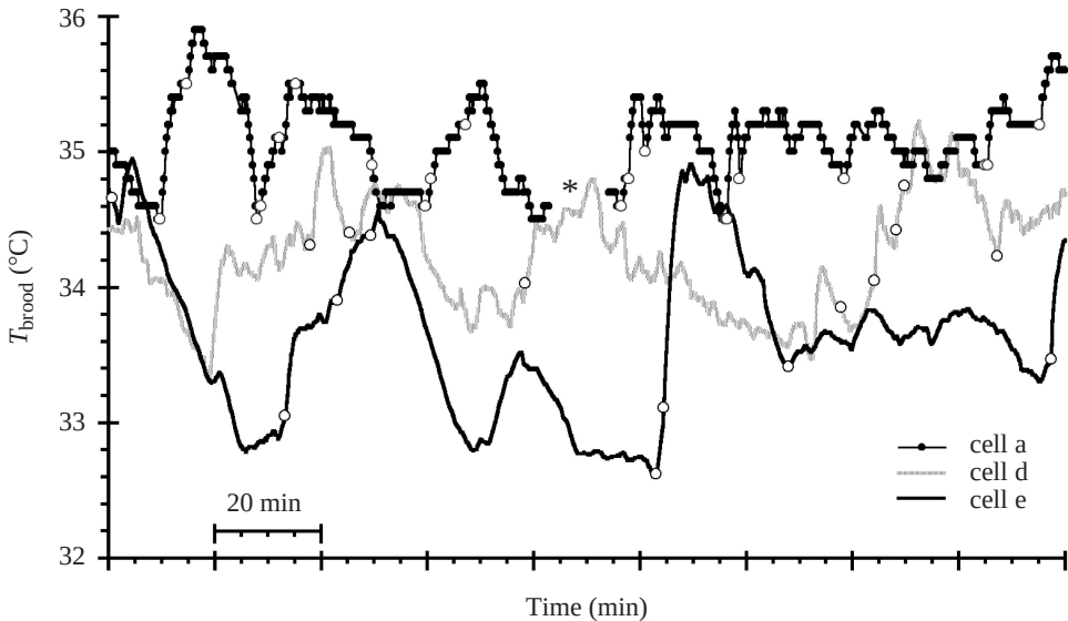
Fig. 8. Interior temperatures of three different brood cells ( T_{brood} ) in an observation hive (setup D), measured simultaneously at the bottom of each cell. All cells were in the same region of the brood nest, 2–3 intermittent cells away from each other, and were adjacent to 4–6 empty cells. Note that cooling and warming may occur simultaneously in different cells. An open circle on the temperature curve marks the time when a bee with a thorax temperature ( T_{th} ) of \geq36^\circ\text{C} entered an empty cell adjacent to this brood cell for a long-duration cell visit ( \geq2\text{ min} ). See Results (setup D) and Discussion for cell visits that are not followed by a temperature change within 2 min and for temperature changes that are not preceded by such a cell visit. Temperatures of cells d and e were stored every second with a resolution of 0.01^\circ\text{C} . The T_{brood} of cell a was read from video every 15 s with a resolution of 0.1^\circ\text{C} (consecutive values are connected by a line for better visualisation of the curve). The asterisk marks a gap of 11 min in the data record of cell a.
