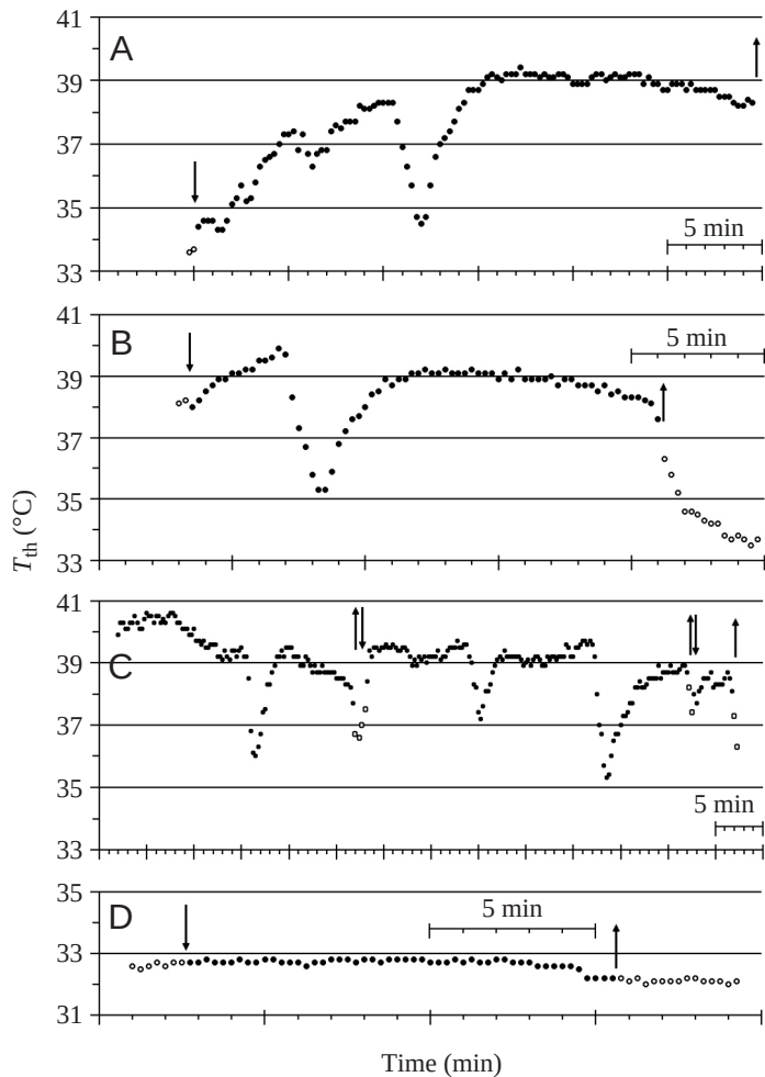
Fig. 6. Thorax temperatures ( T_{th} ) of different honeybees during long visits to empty cells adjacent to sealed brood cells. Bees that are lying still inside cells may be engaged in heat production (A–C) or resting (D). Heating bees with net temperature changes (\Delta T_{th})_{net}=+3.9^{\circ}\text{C} (A) and -0.3^{\circ}\text{C} (B). During a longer cell visit (C), repeated cooling and heating and short interruptions (arrows) occur. Symbols: ↓, bee enters cell; ↑, bee leaves cell. T_{th} of bee outside cell (open circles) and inside cell (filled circles) are plotted.
