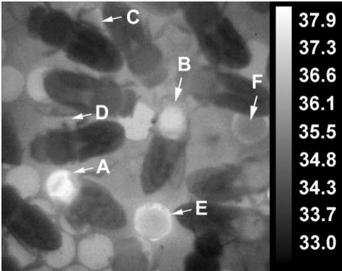
Fig. 5. Thermogram of worker bees in the brood area, as seen in a common observation hive. The sealed area appears grey with no further details in this image; open cells are identifiable by the hexagonal structure of the cell rims. One bee with heated thorax [A; T_{th(entry)}=37.9^{\circ}\text{C} ] is about to enter an open cell adjacent to three sealed brood cells and pokes its head and the anterior part of its thorax into the cell (the dark structure on the heated thorax is the scutellum, seen from posterior-dorsal). Worker bee B has just left the open cell in the centre of the image [ T_{th(exit)}=37.3^{\circ}\text{C} ]. The view on cell visitors C and D is partly hidden by bees on the comb surface. The onset of heat production during cell visits is roughly indicated when the cell interior and thorax (visible as a ring-like structure around the dark silhouette of the cool abdomen) start ‘glowing’ with increasing intensity. Note the different intensities caused by cell visitors E and F.
