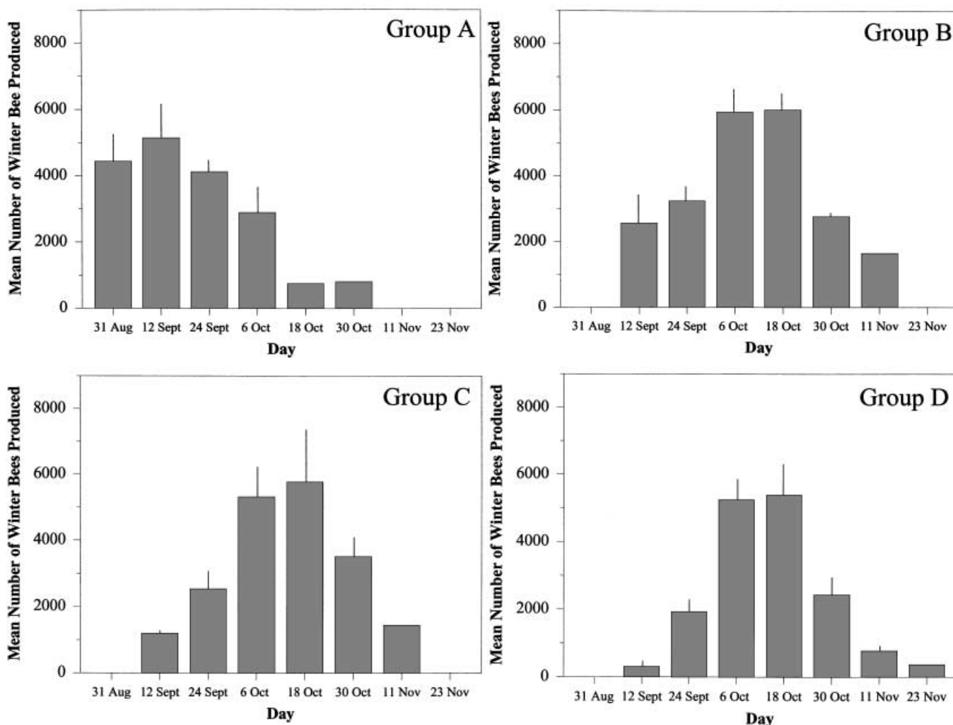
Figure 3. Mean number of winter bees produced ( \pm S.E.) over 12-day intervals until fall brood rearing ceased in colonies receiving one of the following queen treatments: A, original package queen (control); B, requeened with mated queen; C, requeened with virgin queen; or D, made queenless and allowed to rear queen
