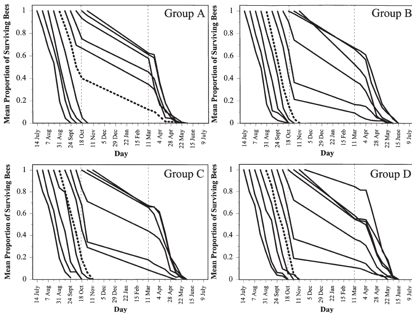
Figure 1. Mean survivorship curves for cohorts of bees introduced at 12-day intervals (from 14 July until fall brood rearing ceased) into colonies receiving one of the following queen treatments: A, original package queen (control, n = 4 ); B, requeened with mated queen ( n = 6 ); C, requeened with virgin queen ( n = 6 ); or D, made queenless and allowed
