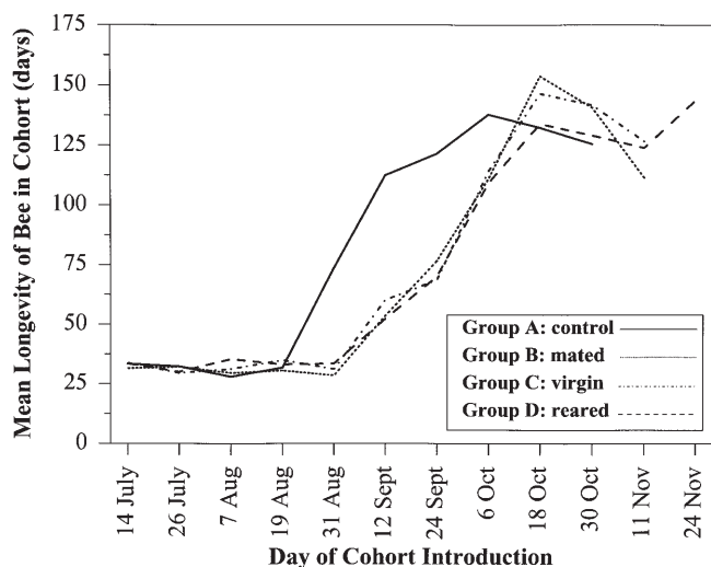
Figure 2. Mean longevity of cohorts of bees introduced at 12-day intervals into colonies left with the original queen (control), requeened with a mated queen, requeened with a virgin queen, or made queenless and allowed to rear a new queen
